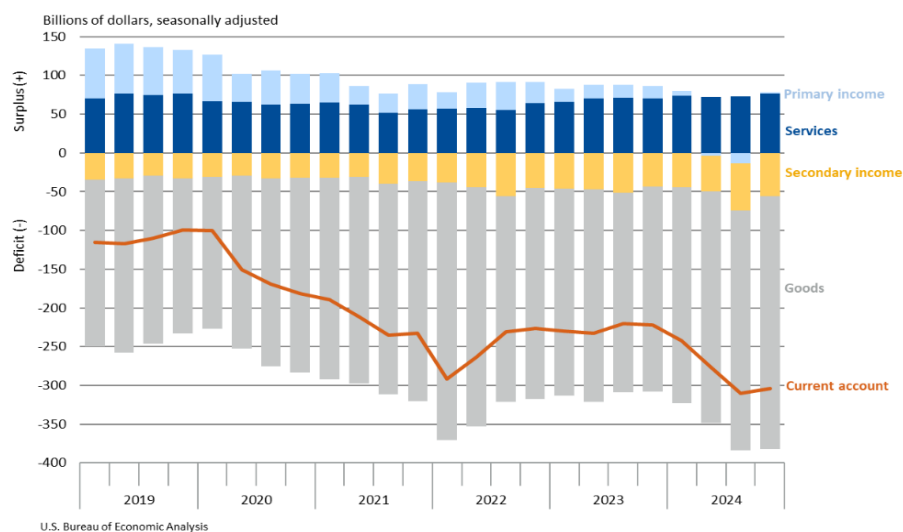
Chart 1. Quarterly U.S. Current-Account and Component Balances
