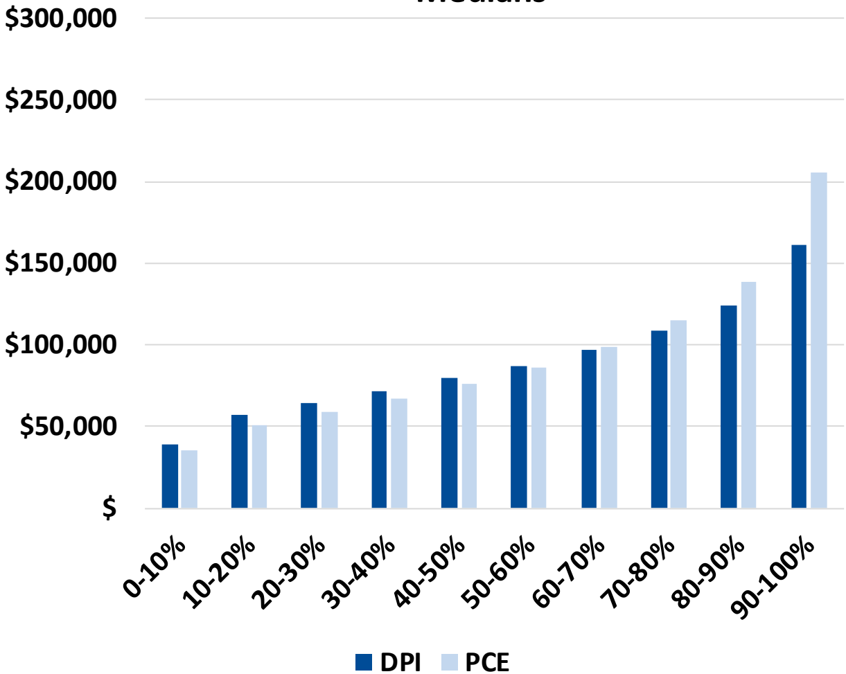
Medians
